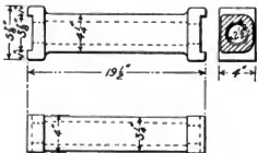
Figs. 3417-3419. Pedestal Brace.
